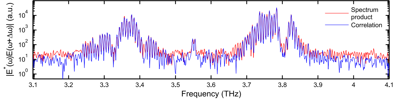
Figure 1: Red line: spectrum product, the product of each laser line and its adjacent line computed from its spectrum. Blue line: correlation product, which represents the same quantity but measured using a fast detector and an analog quadrature technique. Their agreement indicates that the spectrum consists completely of evenly-spaced lines.
