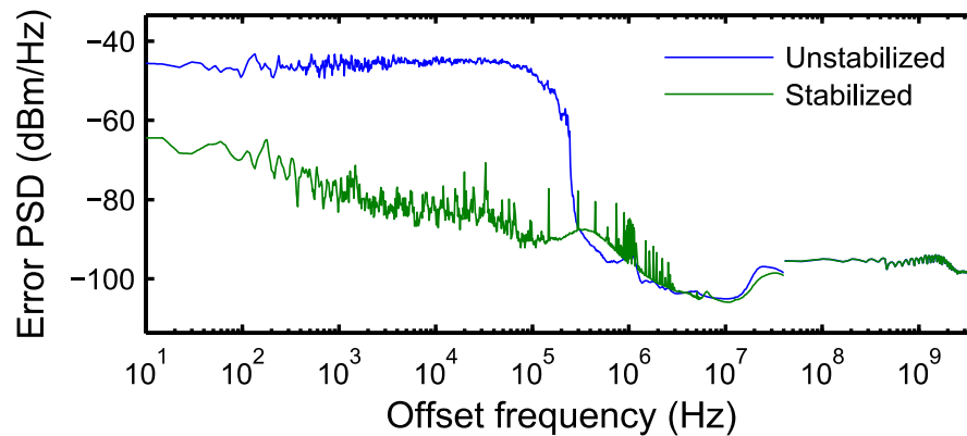
Fig. 1. Beatnote from QCL offset relative to 6.82 GHz, shown with the environmental fluctuations stabilized and unstabilized. 99.92% of the free-running phase noise is removed. (The spectra are discontinuous at 40 MHz because the signal below 40 MHz was measured using downconversion and a fast ADC, while the signal above 40 MHz was measured with an RF spectrum analyzer.)
