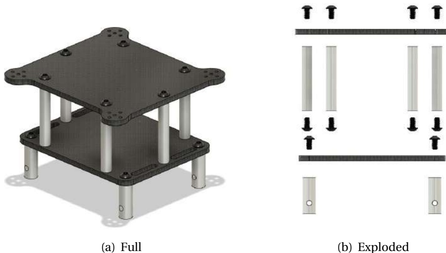
Figure 106: UAV Frame
