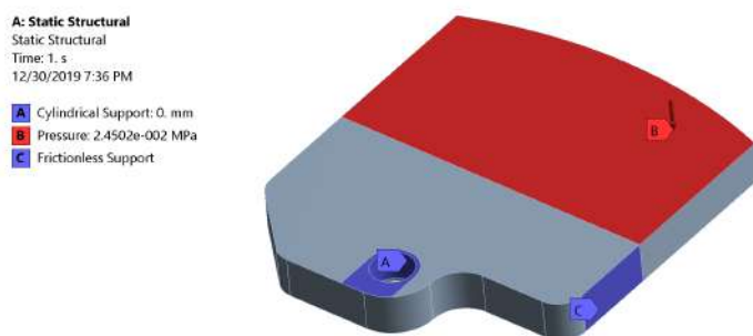
Figure 38: Boundary conditions for drag tab FEA
