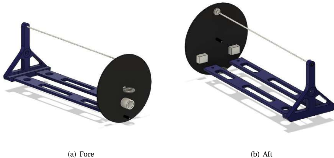
Figure 95: Nose Cone Ejection Assembly
