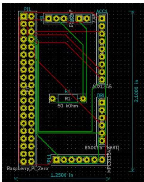
Figure 47: PCB Schematic
