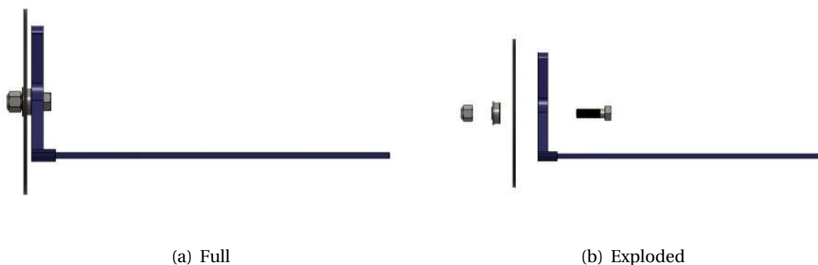
Figure 99: CAD of Orientation System
