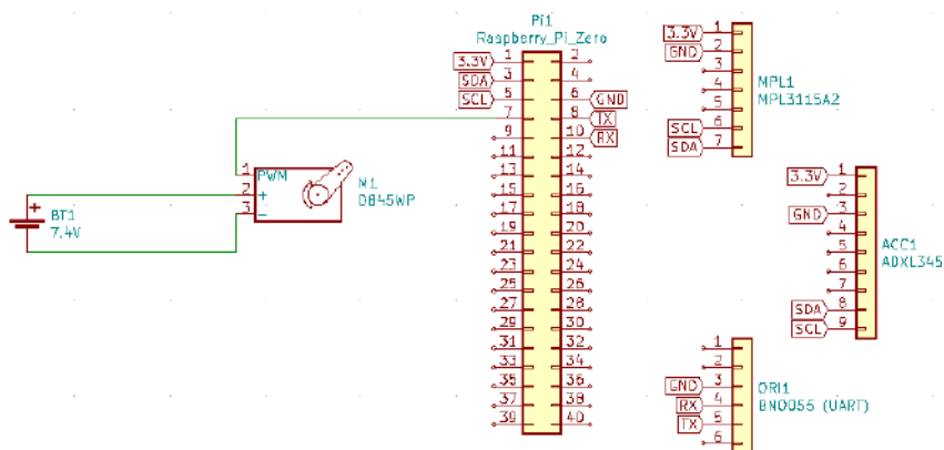
Figure 46: ABS Electronics Wiring Schematic
