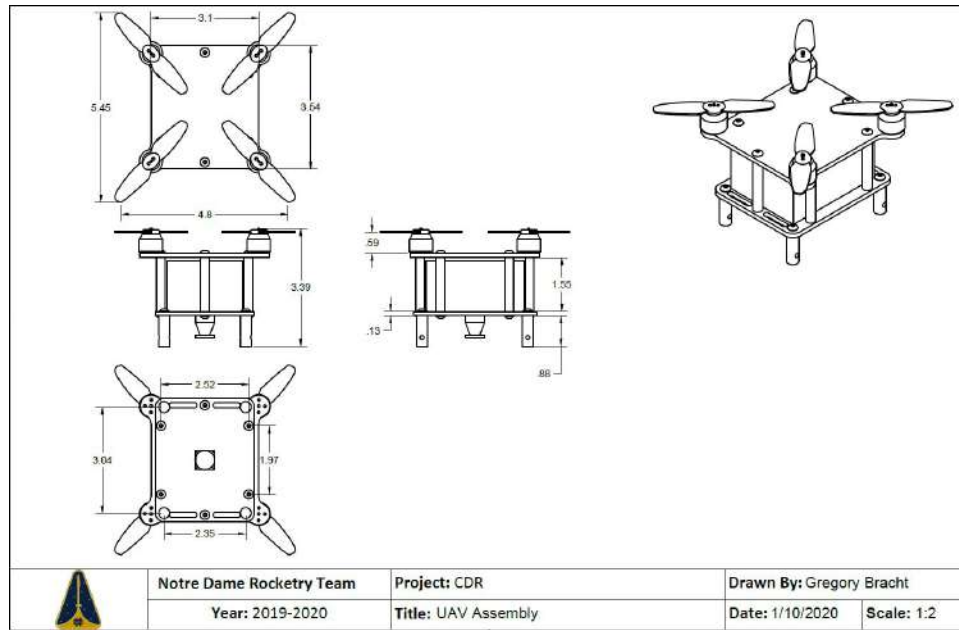
Figure 107: Drawing of UAV Frame
