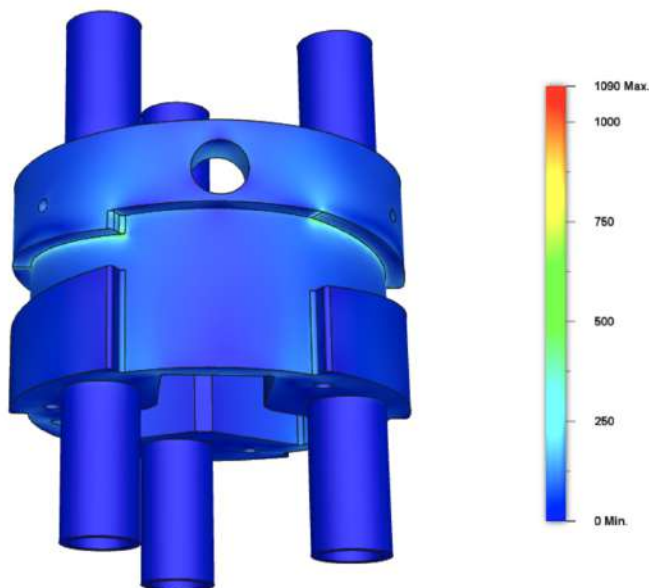
Figure 71: Finite Element Analysis of CRAM body
