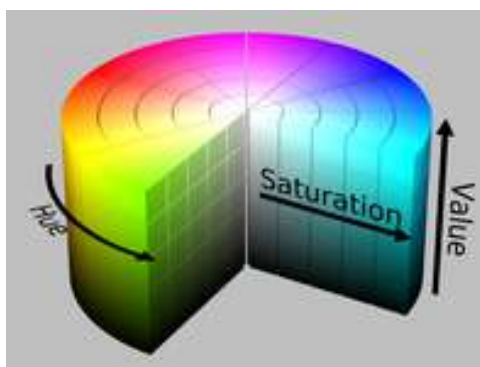
Figure 111: HSV Spectrum.
