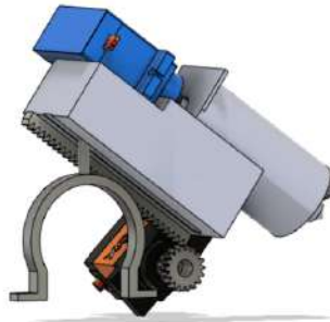
Figure 134: CAD of Sample Retrieval Subsystem
