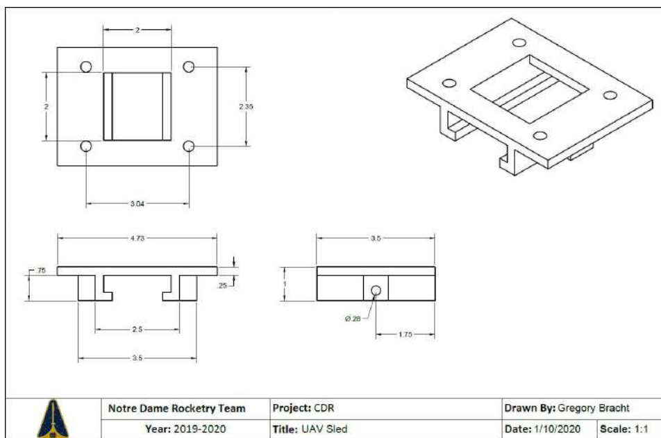
Figure 104: Drawing of UAV Sled
