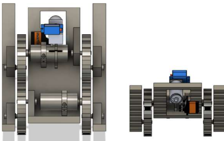
Figure 136: CAD of Archimedes Screw Views
