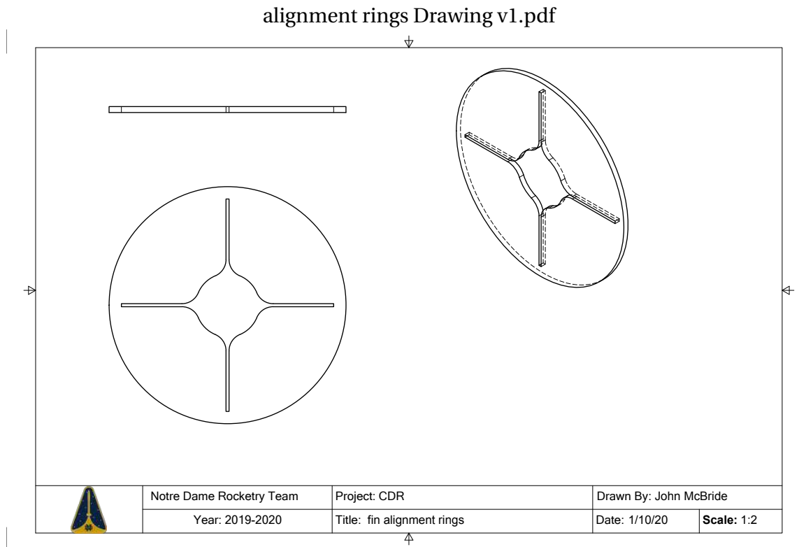
Figure 16: Fin Alignment Rings
