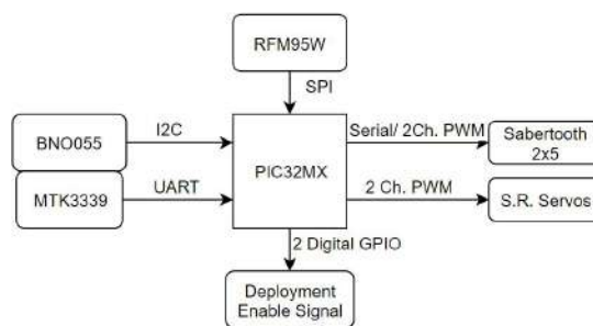
Figure 128: Component Communication
