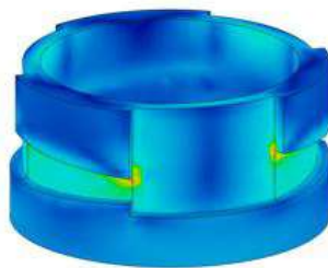
Figure 77: Finite Element Analysis for Stresses in Telemetry Housing Cylinder
