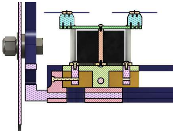
Figure 89: UAV Sled
