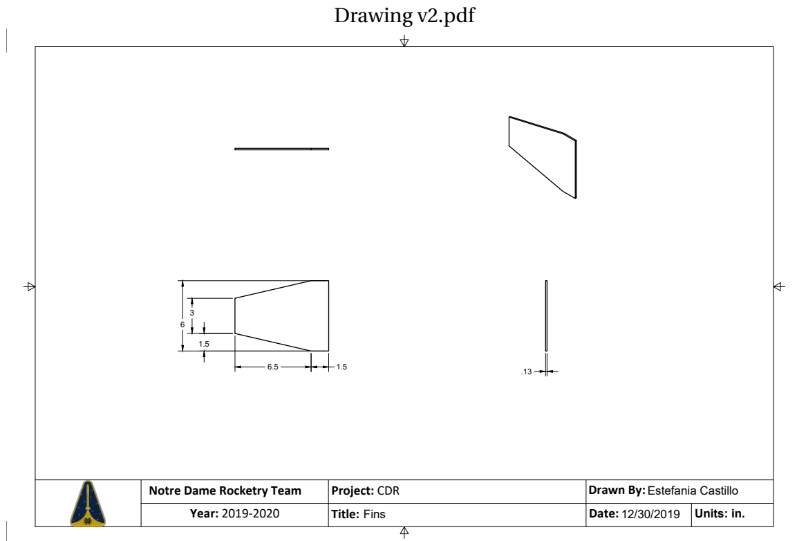
Figure 17: Fin Design and Dimensions
