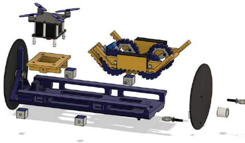
Figure 84: LSRS Exploded View of Vehicle Integration
