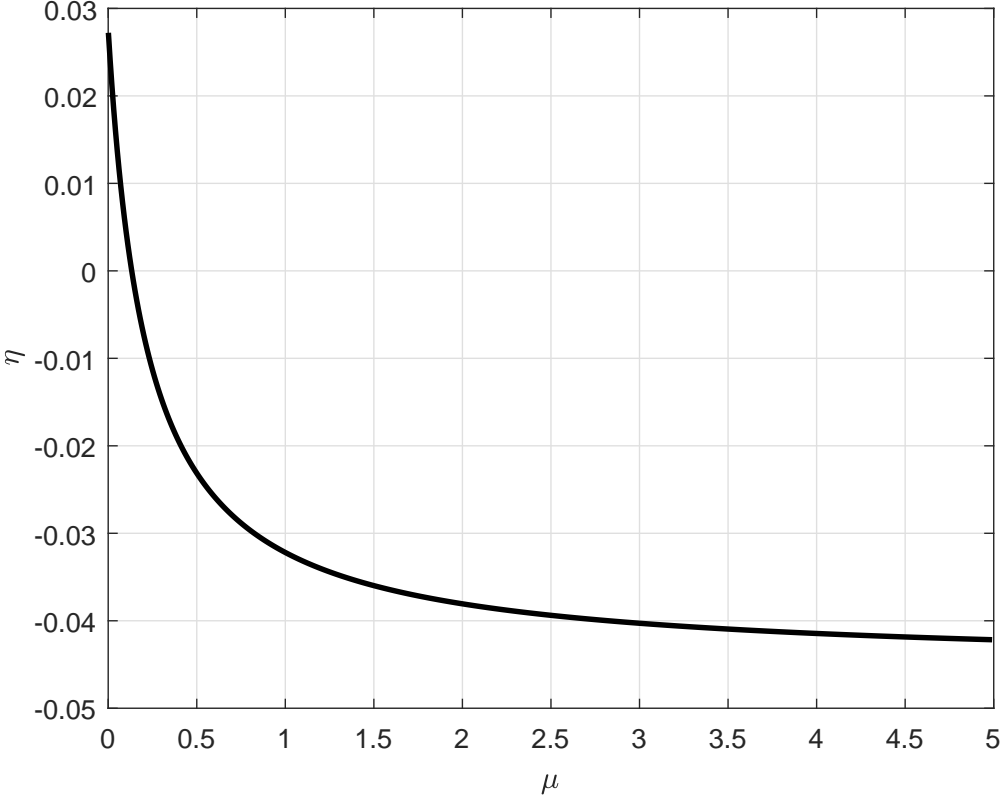
Figure H.3: \eta As a Function of \mu
