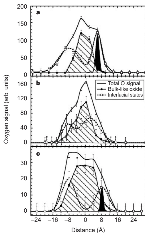
Figure 3 Oxygen bonding profiles from O K edge EELS. The substrate is on the left, and the gate contact is on the right: a , for a c-Si/ \text{SiO}_2 /a-Si stack before annealing (c-Si indicates crystalline Si). The nominal ellipsometric thickness measured after oxidation was 1 \text{ nm} . From EELS, the total O signal has a FWHM of 1.6 \text{ nm} and the bulk-like oxide (hatched area) has a FWHM of 0.85 \text{ nm} . b , After annealing for 10 s at 1,050^\circ\text{C} , the a-Si is converted to polycrystalline silicon, roughening the upper interface. The total O signal has a FWHM of 1.3 \text{ nm} and the bulk-like oxide has a FWHM of 0.85 \text{ nm} . Although the amount of interfacial oxide has not increased, the increased roughness has resulted in an overlap of the two interfacial regions, almost shorting-out the gate oxide (the leakage current is 10 \text{ A cm}^{-2} ). c , In a slightly thicker gate oxide ( 1.8 \text{ nm} ellipsometric thickness), the two interfacial signals no longer overlap and the leakage current is reduced to 10^{-5} \text{ A cm}^{-2} . The total O signal has a FWHM of 2.1 \text{ nm} and the bulk-like oxide has a FWHM of 1.6 \text{ nm} . The inelastic point-spread function, which gives a measure of the probe resolution, is shown as black in a and c .
