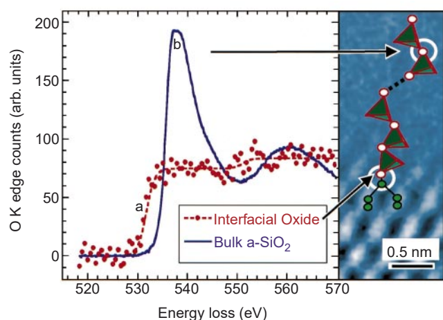
Figure 1 The measured EELS O K edges of bulk a-SiO 2 and for O atoms at an atomically smooth interface between [100]Si and native a-SiO 2 . The 3-eV reduction in the edge onset at the interface aligns the unoccupied O interfacial states with the Si conduction band edge, as would be expected for induced gap states. This pre-peak (a) can be thought of as tunnelling states leaking in from the bulk Si. The reduction in the first bulk peak (b) is discussed in the text. The figure to the right is the annular dark field (ADF) image of the interface between the a-SiO 2 and the silicon substrate. The image is a projection of the ~100 atoms in the path of the beam, so no structural information can be obtained from the amorphous region where the atoms are not aligned along the beam direction. At a rough interface, the bulk lattice would gradually fade into the background over many lattice spacings. The measurements were performed on the Cornell VG-HB501 100 kV STEM equipped with a cold field-emission gun and a McMullan-style parallel EELS spectrometer. The microscope has been modified to achieve high energy-drift stability (<0.2 eV min -1 ) and spatial-drift stability (<0.05 nm min -1 ).
