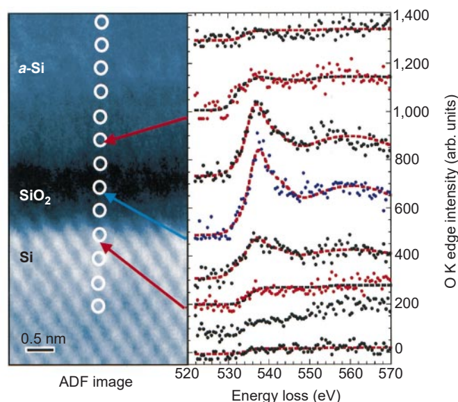
Figure 2 EELS spectra recorded point by point across a gate stack containing a thin gate oxide. The annular dark field (ADF) image (left panel) shows where each spectrum was taken. The [100] silicon substrate is in the lower half, the gate oxide in the middle and the deposited a-Si layer is in top half. The right panel shows the background-corrected O K edges. The smooth curves are the best fits using a mixture of the bulk and interfacial spectra from Fig. 1. The spectra were recorded with a 4-s exposure per point to ensure that the dose was less than the threshold for detectable radiation damage. In growing the gate stacks, particular care was taken to select (using scanning tunnelling microscopy) silicon wafers with exceptionally smooth surfaces before oxidation. The [001] -oriented wafers were cleaned for 15 s in a 15:1 HF solution followed by a 30 s UV-CL clean. The gate oxide was produced by rapid thermal oxidation at 1,000^\circ\text{C} . Chemical vapour deposition (CVD) of a-Si at 550^\circ\text{C} on top of the gate oxide was used as the base of the gate stack, which was subsequently annealed and implanted with dopants. For microscopy, cross-sectioned specimens were dimpled and then ion-milled to electron transparency. The EELS spectra were recorded simultaneously with the ADF signal, under conditions optimized for atomic-resolution imaging 9–12,17 . For a 10-nm-thick sample, the ADF resolution is 0.23 \text{ nm} and the EELS spatial resolution at the O K edge is reduced to 0.26 \text{ nm} due to delocalization 13 .
