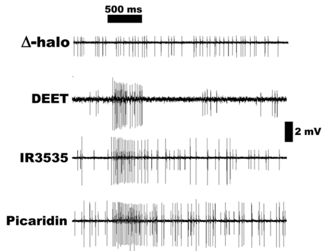
Figure 8. Action potentials recorded from ab3 sensilla. \Delta halo flies showed spontaneous activity of neuron B, but not A, thus showing the ab3A is indeed “empty.” Lower traces were excitatory responses induced by DEET, IR3535, and picaridin and recorded from ab3 sensilla of Or42-expressing flies (w; \Delta halo; UAS-DmOr42a/Or22a-GAL4). doi:10.1371/journal.pone.0017705.g008
