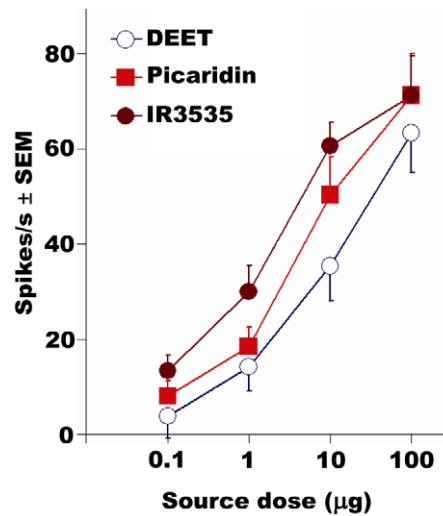
Figure 5. All three insect repellents induce dose-dependent excitatory responses in the pb1A ORN. Hexane (control) responses were subtracted. (N=7). Error bars are standard error of the mean (SEM). doi:10.1371/journal.pone.0017705.g005
