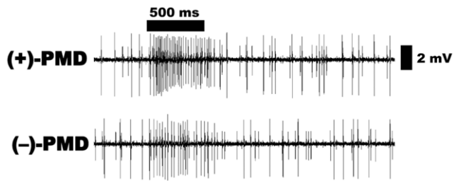
Figure 7. Repellent-sensitive ORN, pb1A, challenged with PMD stereoisomers. (+)-PMD elicited higher response from the large spike neuron than (-)-PMD. Source dose, 100 \mu g. doi:10.1371/journal.pone.0017705.g007
