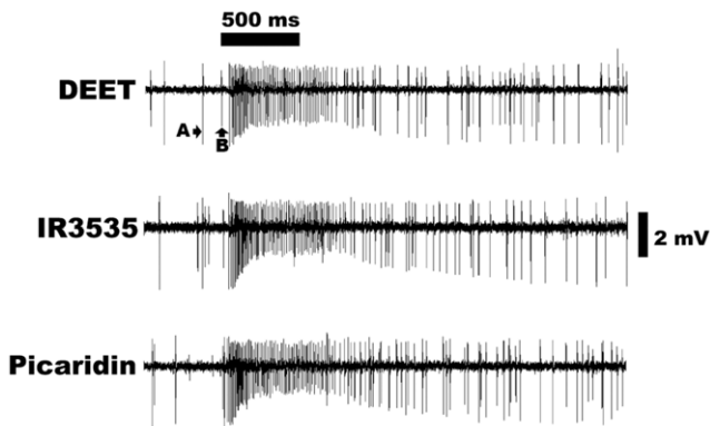
Figure 4. Excitatory responses from an ORN housed in the maxillary palp basiconic sensillum pb1A when challenged with three insect repellents: DEET, IR3535 and picaridin. Two types of neurons, A and B, are identified on the basis of their spike amplitudes. The ORN with larger amplitude, A, is stimulated by the three insect repellents, whereas the neuron with smaller amplitude, B, was unresponsive. Source dose, 100 \mu g. doi:10.1371/journal.pone.0017705.g004
