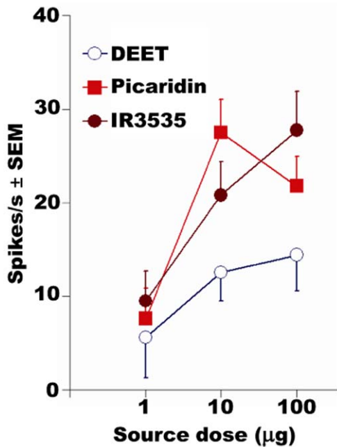
Figure 10. Dose-dependent responses from ab3A neuron of transgenic flies expressing Or42a (w; \Delta halo; UAS-DmOr42a/Or22a-GAL4). Test flies were challenged with DEET, IR3535, and picaridin ( N=15 ). Error bars are standard error of the mean (SEM). doi:10.1371/journal.pone.0017705.g010
