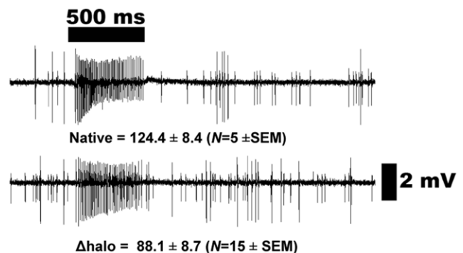
Figure 9. Comparative responses of Or42a expressed in its native environment and in the “empty neuron.” Ethyl butyrate (source dose, 10 \mu g) elicited higher responses from pb1 sensilla of wild type flies (top trace) than from the ab3 sensilla of Or42a-expressing flies (w; \Delta halo; UAS-DmOr42a/Or22a-GAL4) (lower trace). SEM, standard error of the mean. doi:10.1371/journal.pone.0017705.g009
