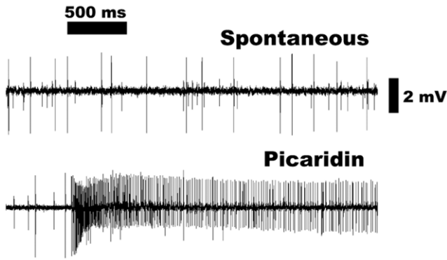
Figure 3. Extracellularly recorded single unit responses from an ab3 sensillum. Spontaneous activity (upper trace) and picaridin-induced excitatory response (lower trace) from the large amplitude neuron, ab3A. Source dose, 100 \mu g. Note the excitatory responses lasted beyond the stimulus period. doi:10.1371/journal.pone.0017705.g003
