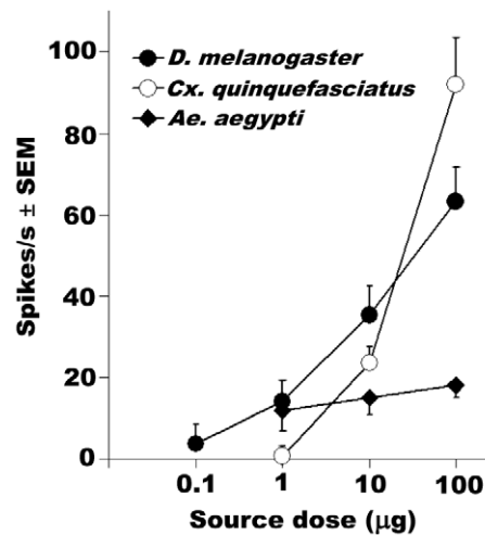
Figure 6. Comparative DEET-elicited responses. DEET-induced excitatory responses from Drosophila pbA1 ORN showed lower threshold than those recorded from the DEET-sensitive mosquito ORNs from the Southern House mosquito, Cx. quinquefasciatus [20] and the yellow fever mosquito, Aedes aegypti [21], respectively. Error bars are standard error of the mean (SEM). doi:10.1371/journal.pone.0017705.g006
