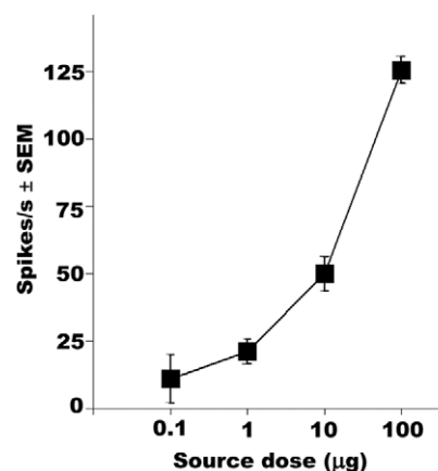
Figure 2. Dose-dependent excitatory responses from a picaridin-sensitive ORN housed in an antennal basiconic sensillum ab3 on D. melanogaster antennae. Hexane (control) responses were subtracted. ( N=7 ). Error bars are standard error of the mean (SEM). doi:10.1371/journal.pone.0017705.g002
